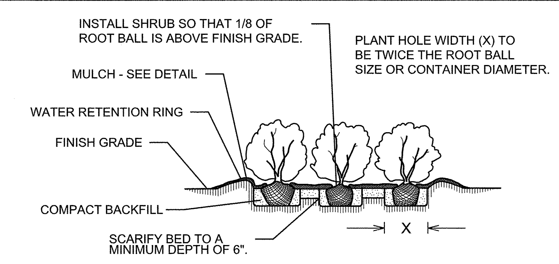
GROUND COVER/ BEDDING PLANT DETAIL SHRUB BED PLANTING DETAIL
