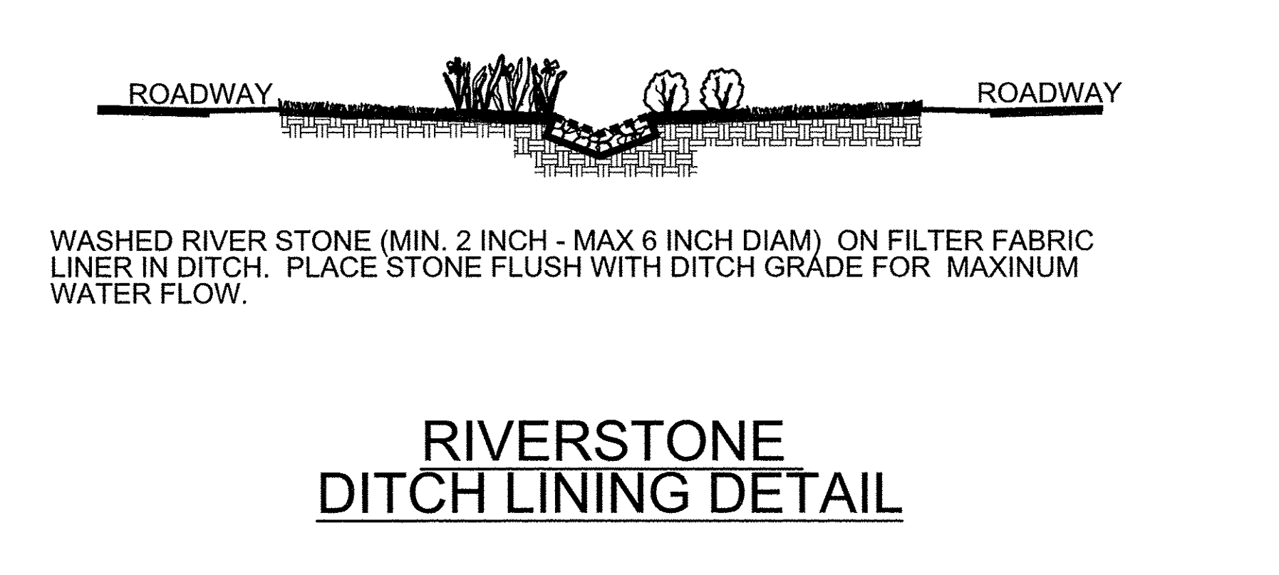
RIVERSTONE DITCH LINING DETAIL
