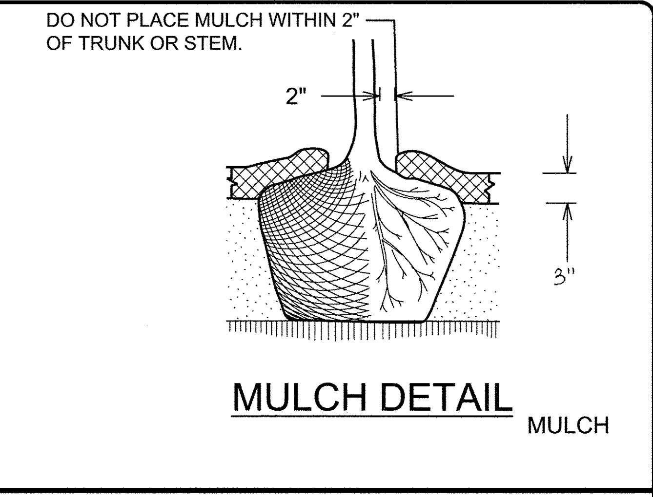
MULCH DETAIL
